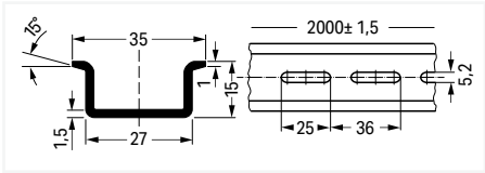
Steel DIN-rail ▶ I N 125 A (based on 1 m length) ▶ 35 x 15 mm ▶ 1.5 mm thick ▶ 2 m long ▶ per EN 60715
