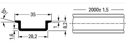
Aluminum DIN-rail ▶ I N 76 A (based on 1 m length) ▶ 35 x 8.2 mm ▶ 1.6 mm thick ▶ 2 m long ▶ similar to EN 60715
