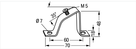
Angled support bracket ▶ without screw
