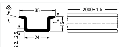
Copper DIN-rail ▶ I N 309 A (based on 1 m length) ▶ 35 x 15 mm ▶ 2.3 mm thick ▶ 2 m long ▶ per EN 60715
