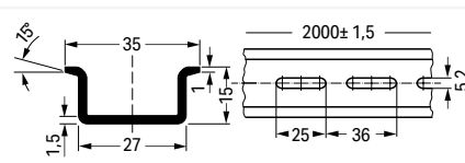
Steel DIN-rail ▶ I N 125 A (based on 1 m length) ▶ 35 x 15 mm ▶ 1.5 mm thick ▶ 2 m long ▶ similar to EN 60715
