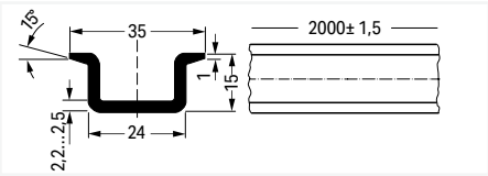
Carrier rail ▶ plastic Not suited for use with ground terminal blocks!
